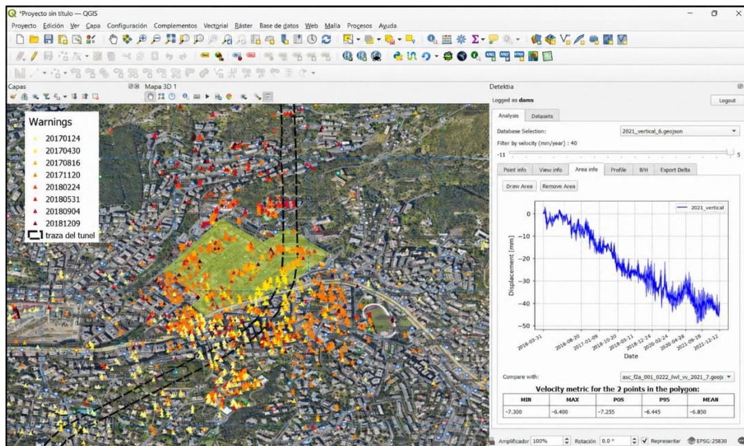
Figure 7 Detektia's InSAR outputs integrated into a desktop GIS environment, with date-coded deformation warnings and velocity statistics for a user-selected polygon. Source: Detektia
