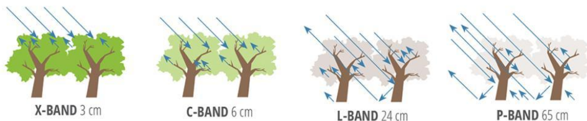
Figure 3 Sensitivity of SAR measurements to forest structure and penetration into the canopy at different wavelengths used for airborne or spaceborne remote sensing observations of the land surface. Credit: NASA SAR Handbook.
