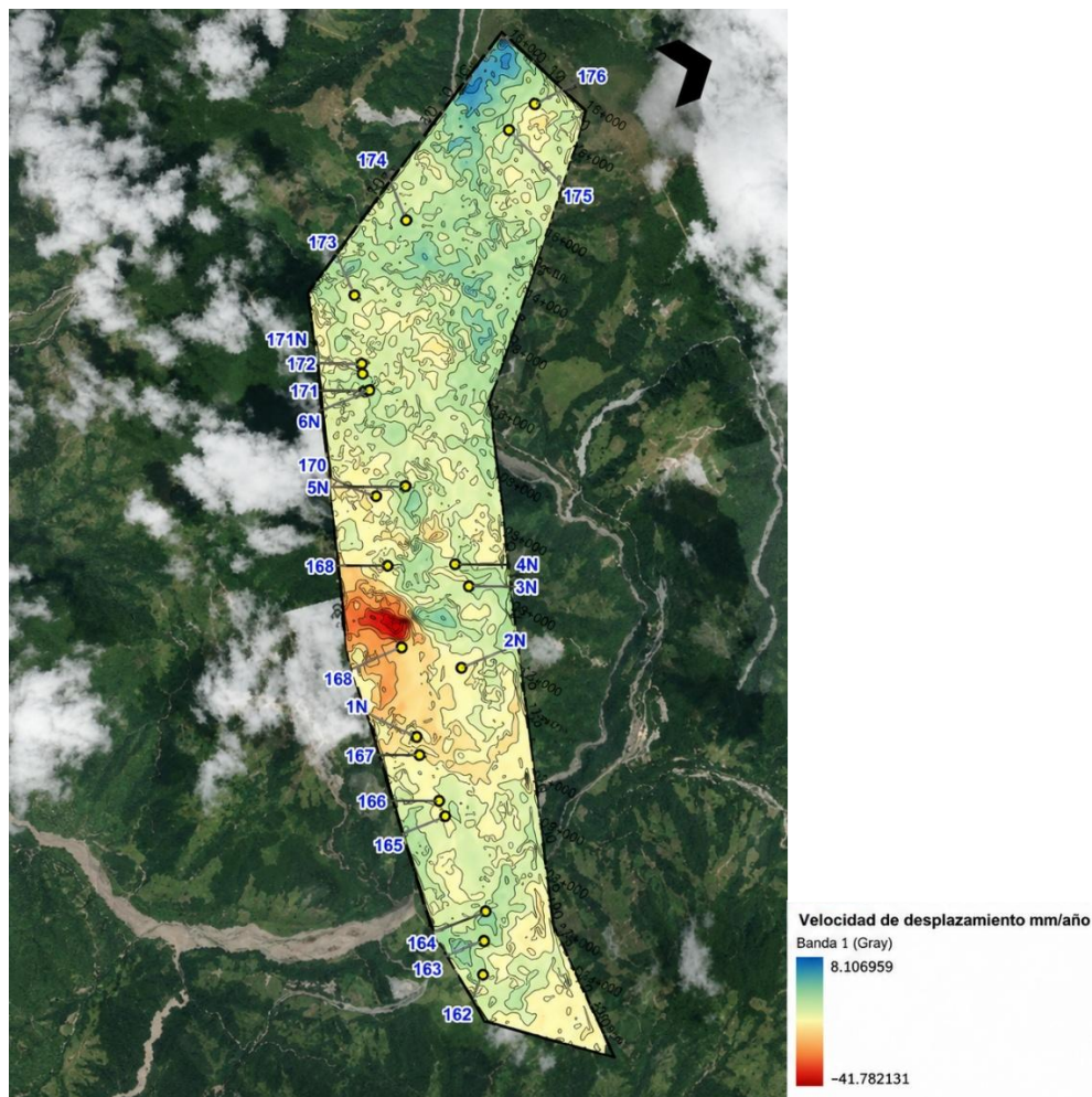
Figure 17 InSAR-derived deformation along a monitored slope, colour-coded by displacement; the concentration of movement is what directs field inspection. Source: Geoandina-i SAS
