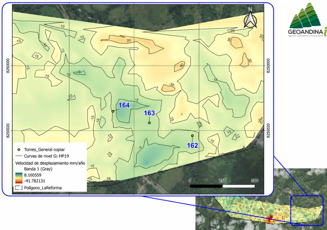
Figure 13 Processed terrain and geotechnical analysis of a monitored area. Source: Geoandina-i SAS.
